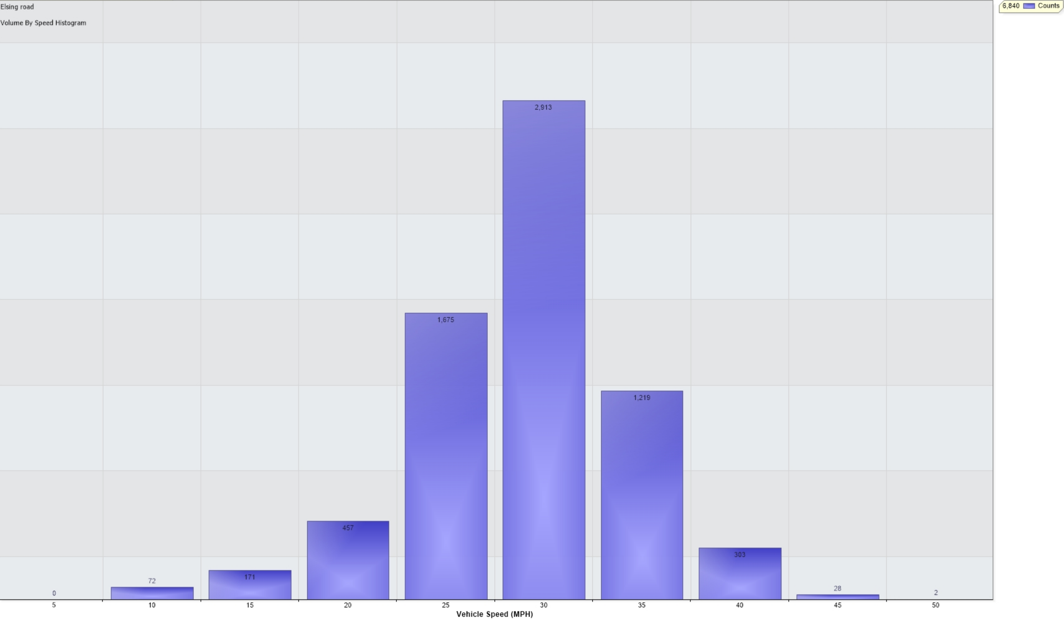
Vehicle Counts Vs. Speed [Elsing road: Incoming]
