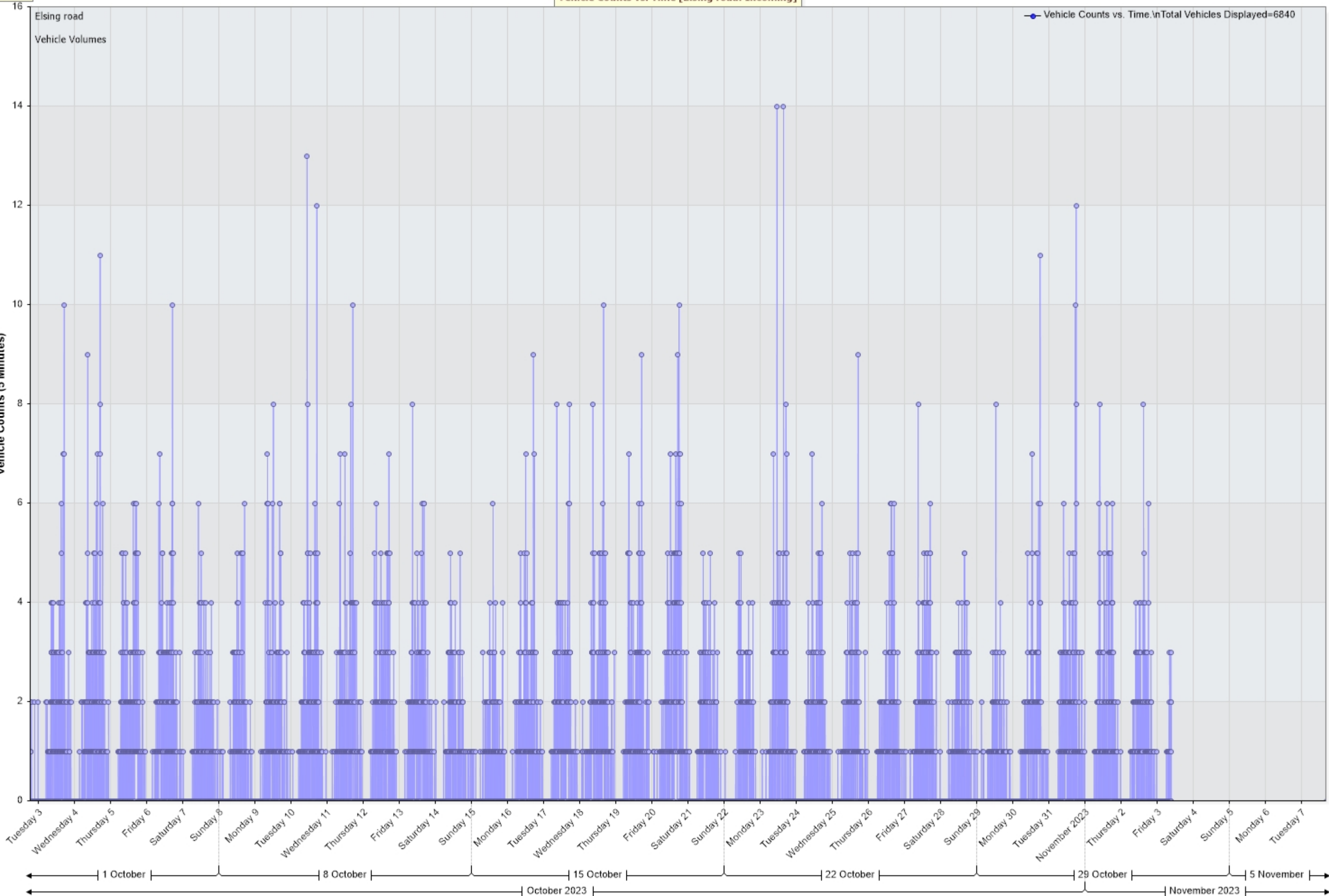
Vehicle Counts vs. Time [Elsing road: Incoming]
